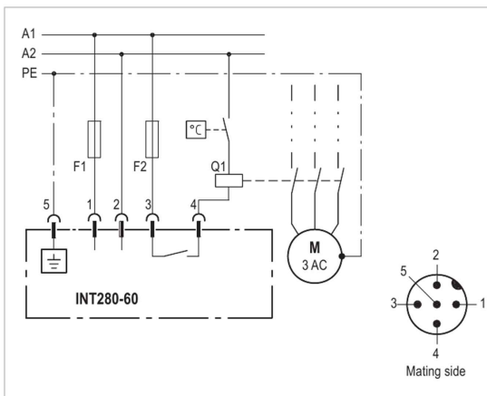
Wiring diagram
