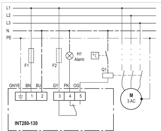
Wiring diagram
